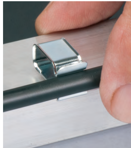
Snap one or two USE-2 or PV cables securely in place.
