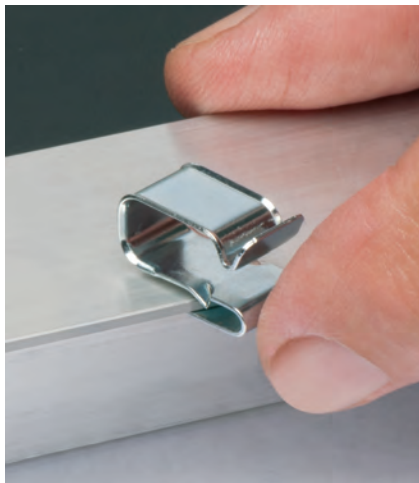
Snap Wire Clip onto sheet metal up to .080" thick.
