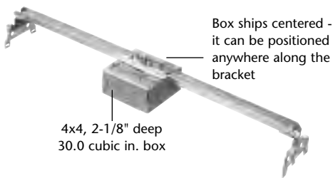
2 FS427SCL is shipped ready for a centered installation on the ceiling grid. Position ends of support bar over the ceiling grid (tees).
