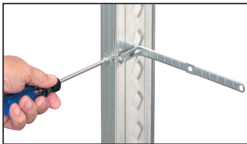
1 Nail or screw CUS6 support to metal or wood stud (metal shown).
