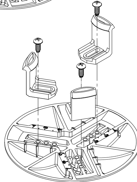
ISOMETRIC ASSEMBLY VIEWS
