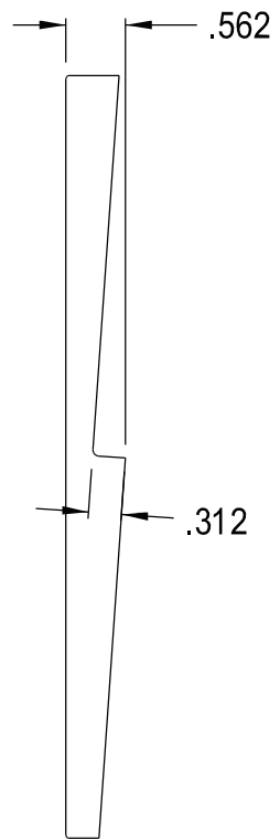
DBVR131 1/4" & 5/16" LAP
