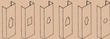
Common hole configurations in metal studs.
