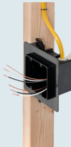
Installer must caulk around cable when it's installed to meet NEMA OS-4 requirements
