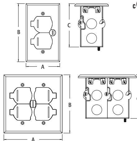
FLB5551MB
