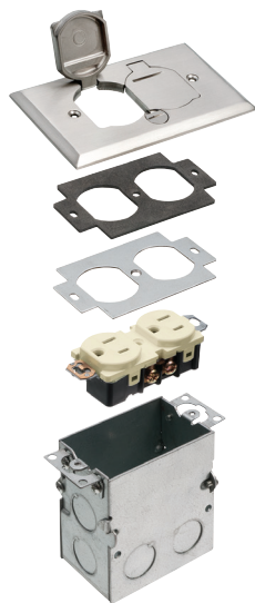
FLB5331NL
