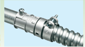
3/4" EMT to 2411 to L422 with flexible metal conduit
